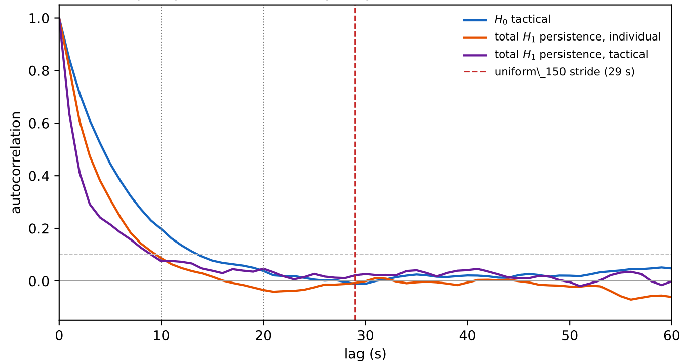
Topological summaries, Sydney FC vs Adelaide United (1 Hz)
